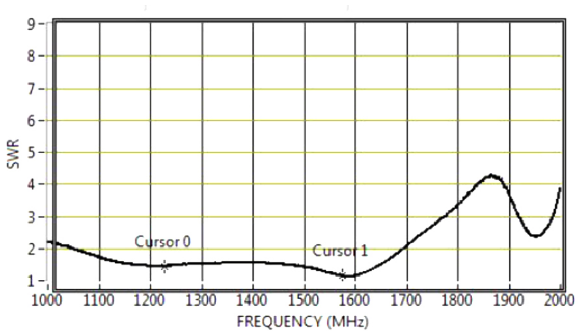
Figure 2-2. Passive MS14 Splitter: SWR vs. Frequency
