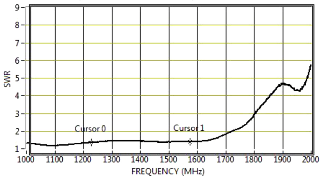
Figure 2-4. Active MS14 Splitter: SWR vs. Frequency
